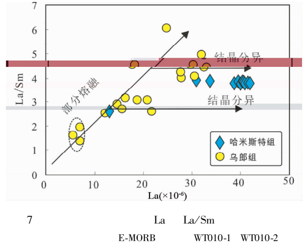
7 La La/Sm E-MORB OIB WT010-1 WT010-2 WT012-1 Fig. 7 La vs. La/Sm of the Nileke Permian volcanic rocks
