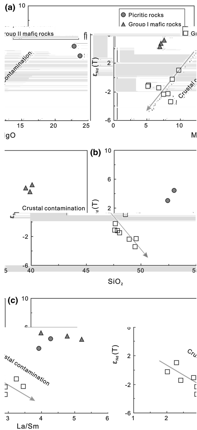
Fig. 9 Plots of \epsilon_{\text{Nd}}(T) versus \text{MgO} , \epsilon_{\text{Nd}}(T) versus \text{SiO}_2 , and \epsilon_{\text{Nd}}(T) versus \text{La/Sm} for the Datian mafic–ultramafic dykes
