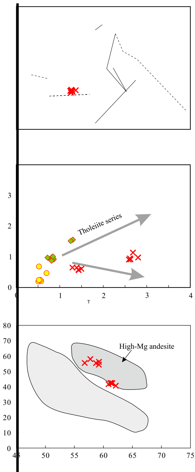
Figure 9. (A) Incompatible elements (Zr/Ti vs. Nb/Y) classification diagram; (B) \text{TiO}_2 (wt%) vs. \text{FeO}/\text{MgO} (wt%) plots for discrimination between the calc-alkaline and tholeiitic series (Miyashiro 1974); (C) Mg# vs. \text{SiO}_2 (wt%) classification diagrams for the Dawan high-Mg andesites.
